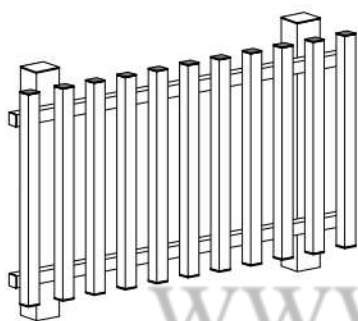
1 Square profile 20x20mm Profilé caré 20x20mm
